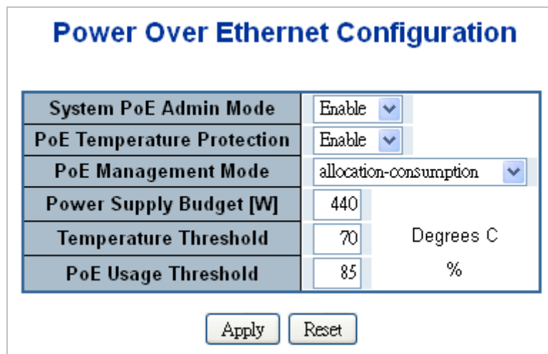
Figure 4-16-2: PoE Configuration Screenshot
